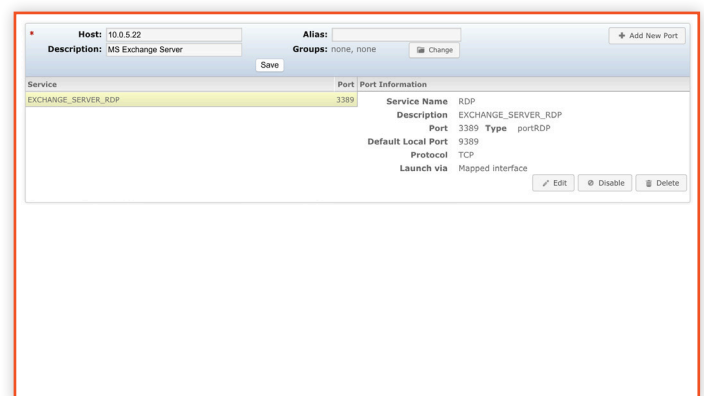
SecureLink GUI
